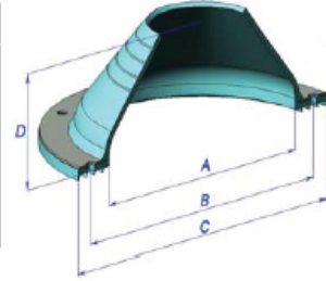
Standard-PIPETITE PT(70-135), PT(100-180)
